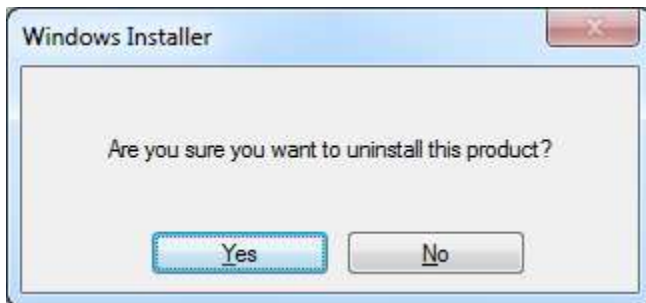
Fig C.2.1. Confirmation panel
