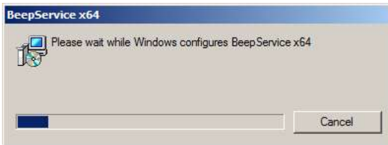
Fig C.2.6. Uninstall progress
