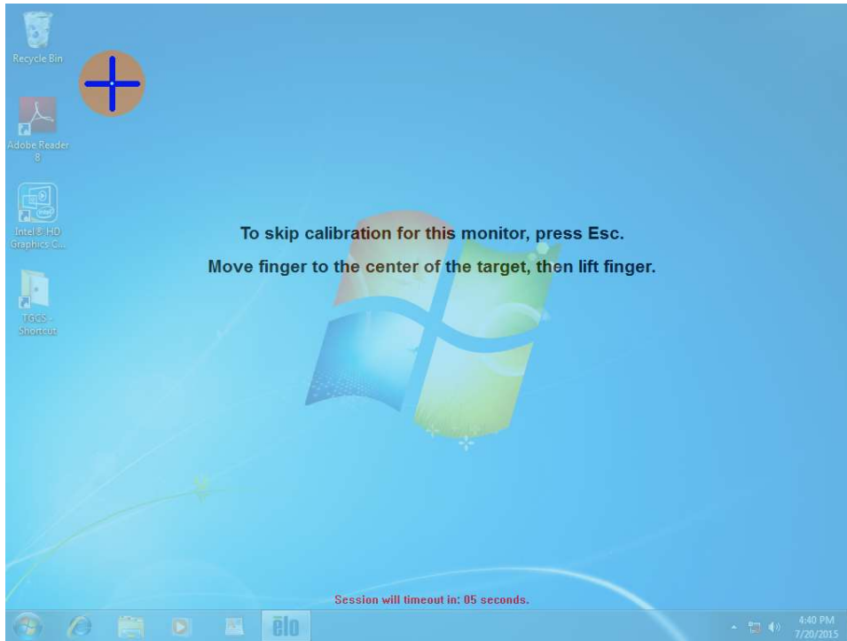
Fig C.1.5. Calibrate/Associate target
