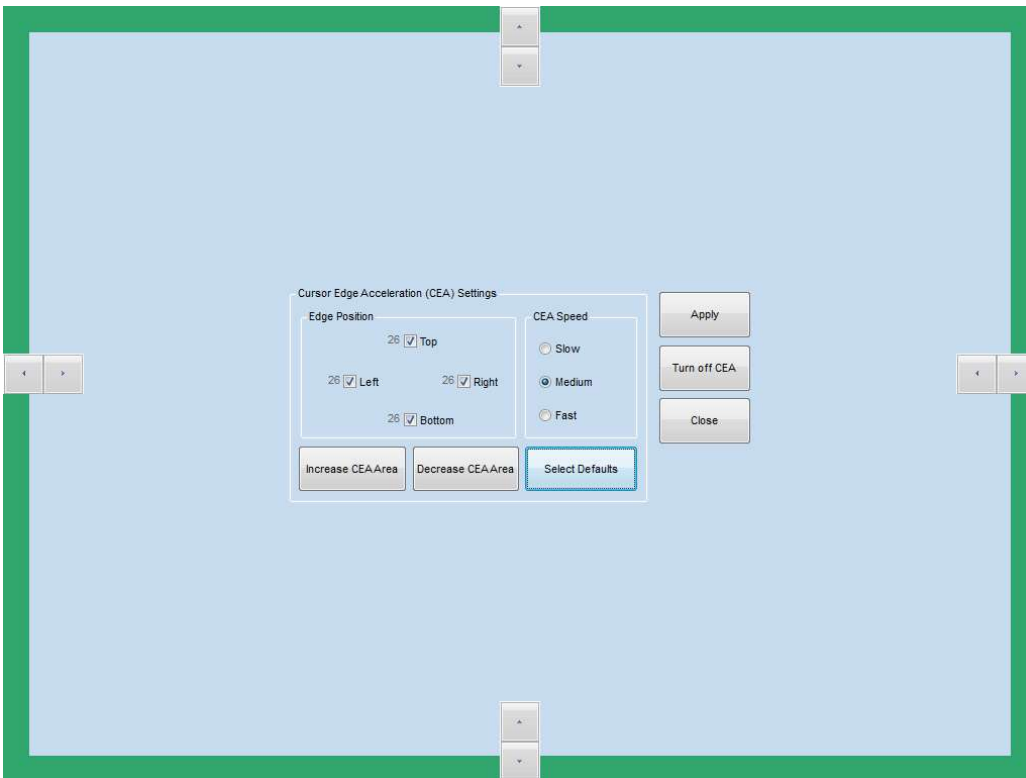
Fig C.1.10. CEA adjustments
